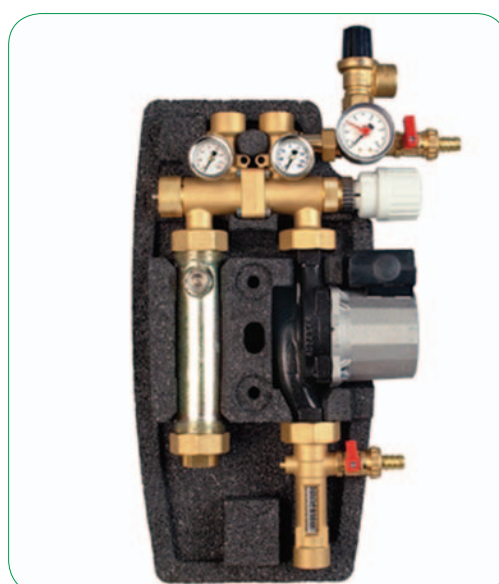
Solar Station Dual Line
